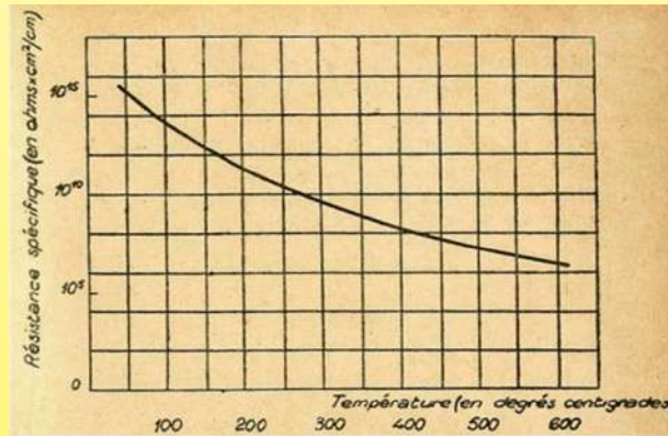
Variation of the specific resistance in ohms.cm/cm 2 of the porcelain according to the temperature (logarithmic curve). Between 20 °C and 300 °C its resistance is divided by 10,000 (1945 Matériaux électrotechniques modernes, Ultimheat Museum)
